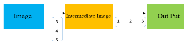
Separable CNN
