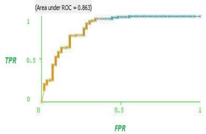
RBF
